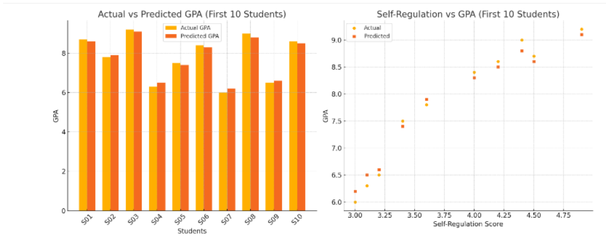
Fig 2: Actual Vs Predicted GPA for 10 Students
