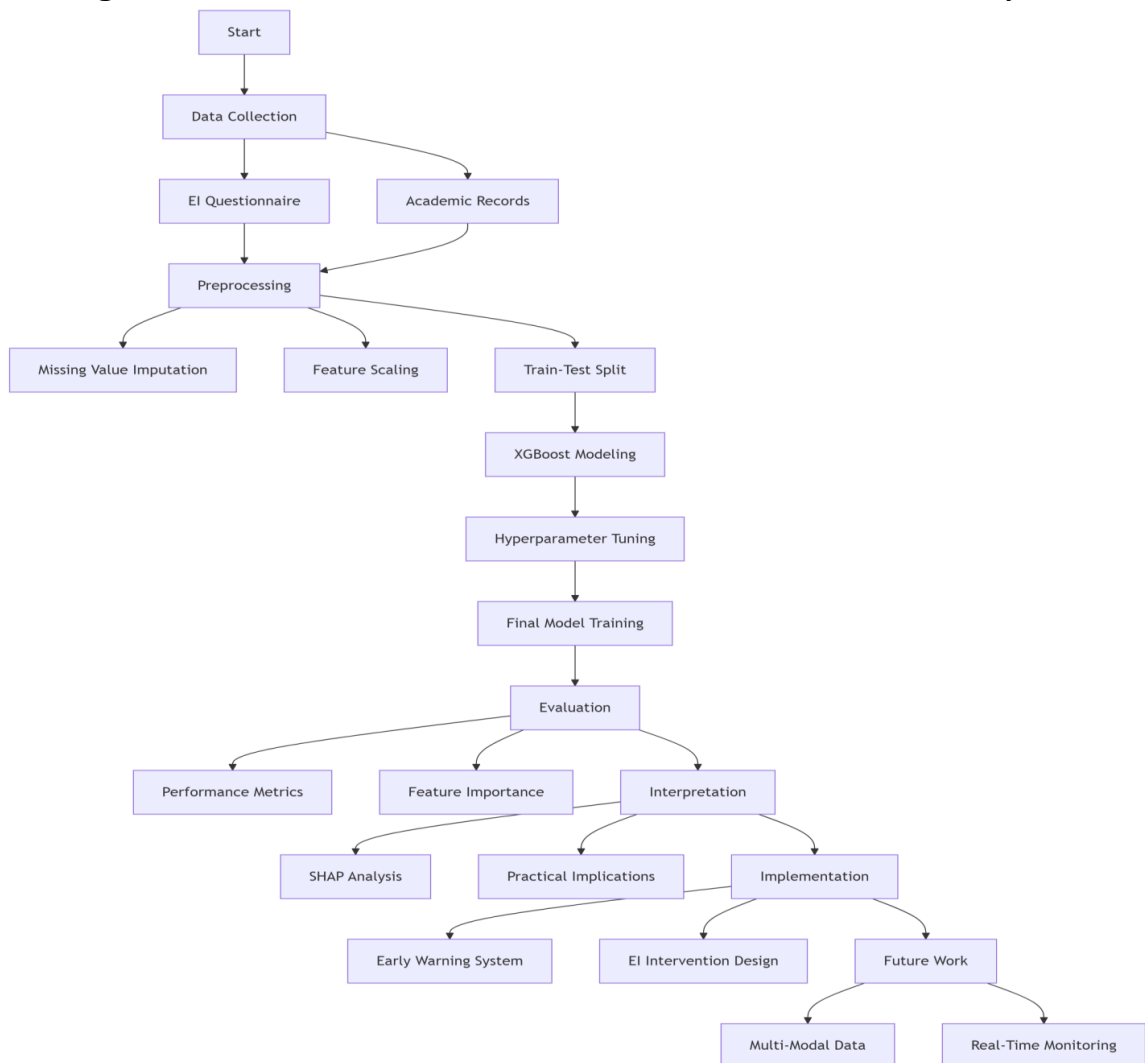
Fig 1: Architectural Overview of the EI-Academic Performance Prediction System
