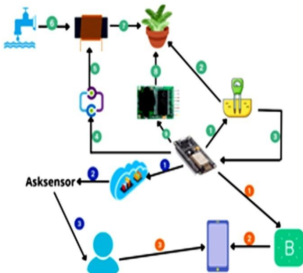
Figure 2: Block Diagram of IoT based Smart Agriculture Water Level Sensor (optional) used to monitors available water in tanks or reservoirs. Microcontroller Setup Used to NodeMCU ESP8266 sensor (or) ESP32 for sensor data acquisition and internet connectivity. It is programmed using Arduino IDE.
