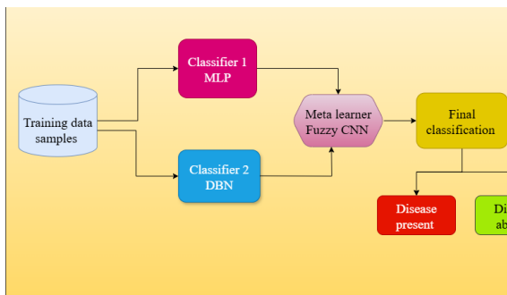
Fig 2 Structure of stacked ensemble classifier
