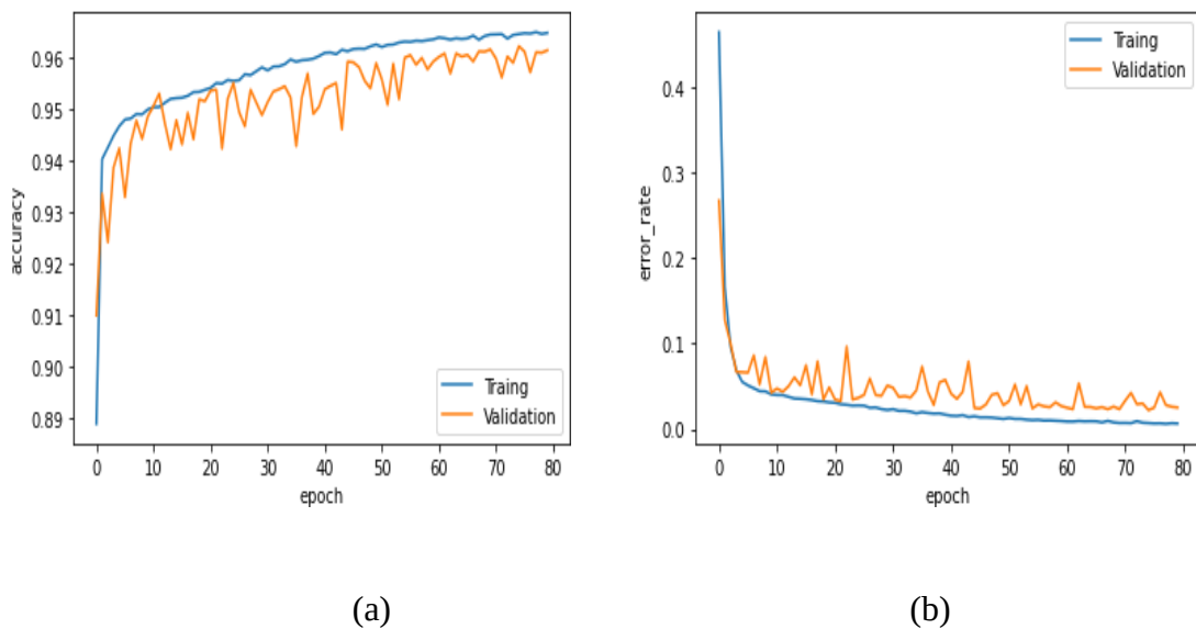
Figure 6. Learning curves of the proposed RRUNC Model, a) Accuracy curve, b) Error rate curve
